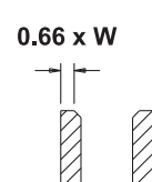
DIN 1838BW PARROT FORM TOOTH WITH ALTERNATE BEVEL
